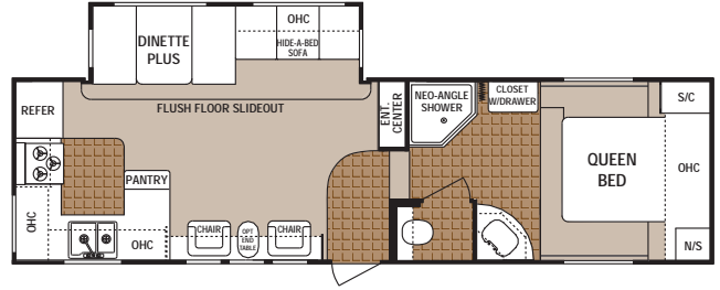
28RK-M5
